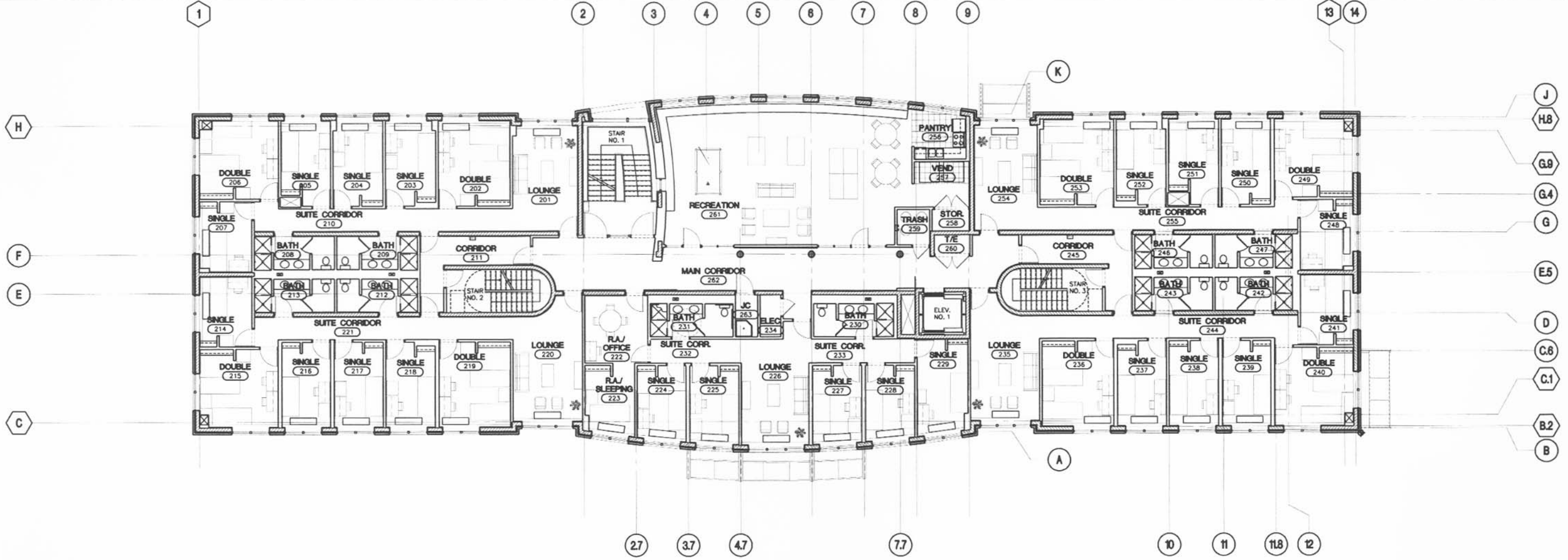
Second Floor Furniture Plan SCALE: 1/8"=1'-0"
